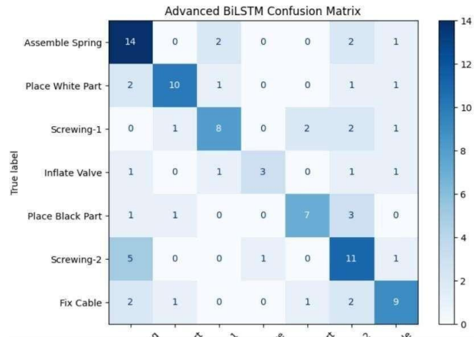
Fig.8.8 Confusion Matrices
